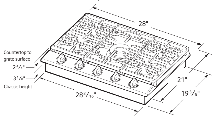
Cooktop Dimensions
