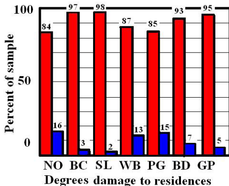
Figure 10. Normalized percentage of wind damage to residences for the seven geographic zones in the study area. Red bars are DOD 2 or less whereas blue bars are DOD 4 or more.
