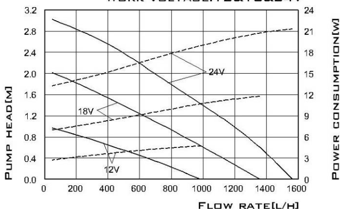
PUMP CURVE
