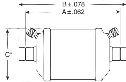
*DOES NOT INCLUDE WELD BEAD
