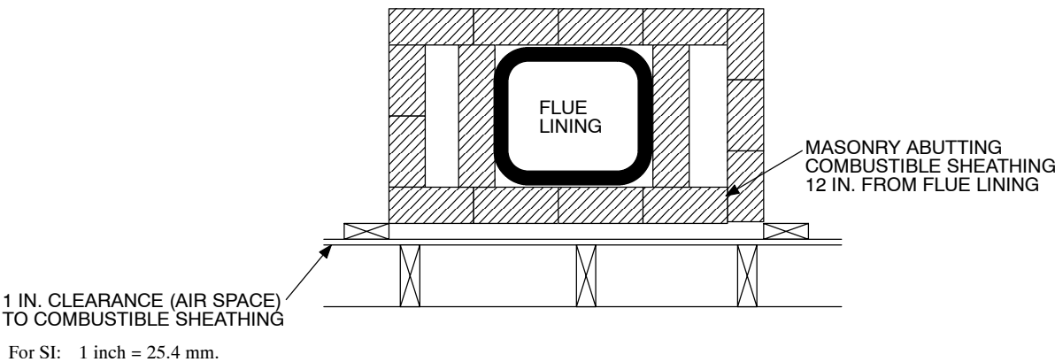
FIGURE R1001.15 CLEARANCE FROM COMBUSTIBLES
