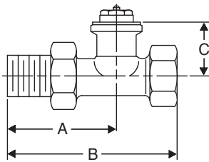
RV-4 Straight
