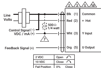
Proportional, CQKB24-SR-LR
