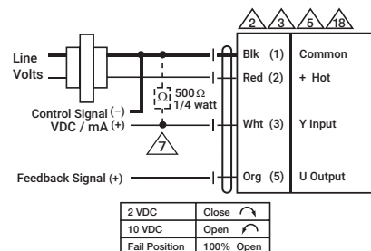
Proportional, CQKB24-SR-RL
