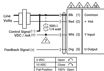
Proportional, CQKB24-SR-LL
