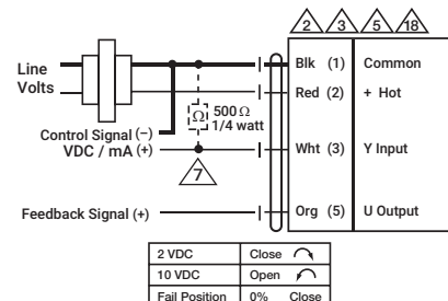
Proportional, CQKB24-SR-RR
