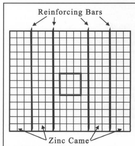
Figure 6. The four vertical reinforcing bars were soldered to the inside face of the transom panel. Drawing: Chad Randl.
