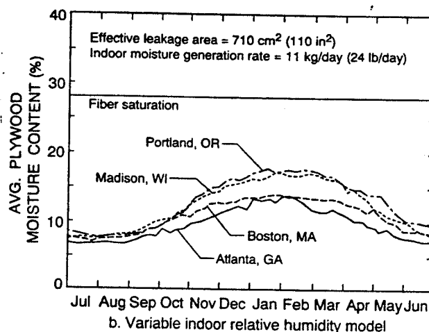
Figure 1 Effect of climate on plywood moisture content.
