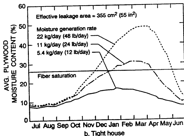
Figure 5 Effect of moisture generation rate in Madison, Wis.
