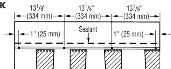
Figure 15-3: Use four nails for every full shingle.
