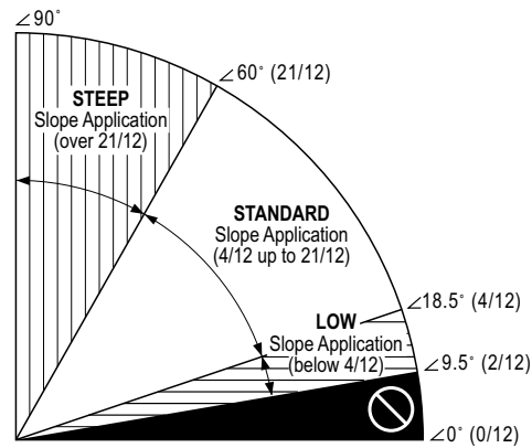
Figure 12-1: Slope definitions.
