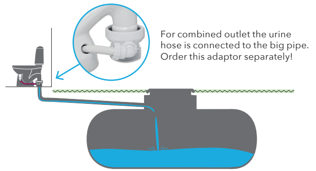
Combined outlet
