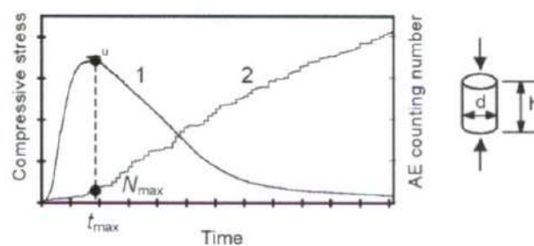
1 - Compressive stress 2 - AE counting
