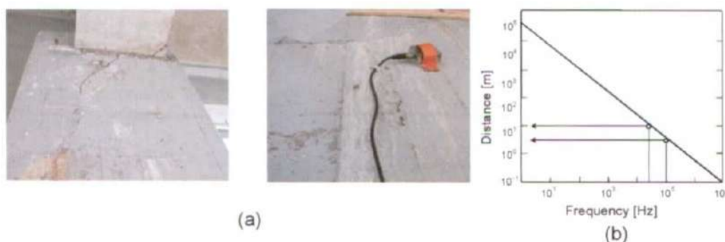
Fig. 3 : Cracks in the P_1 pier and the applied sensor (a). Relationship between signal detection distance and signal frequency (b).
