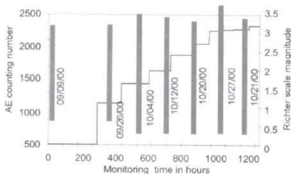
Fig. 7: AE and seismic events
