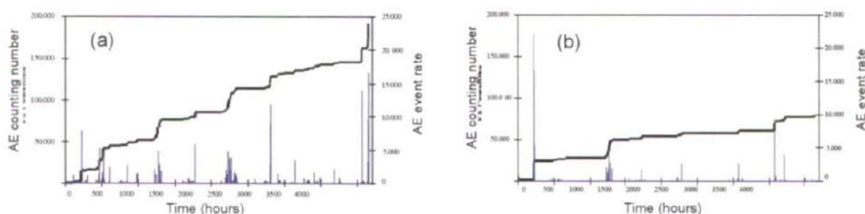
Fig. 4: Piers P_1 (a) and P_2 (b) monitoring data
