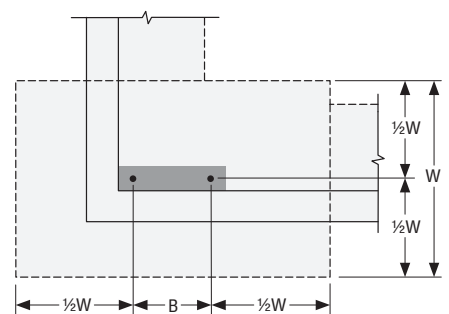
Footing Plan
