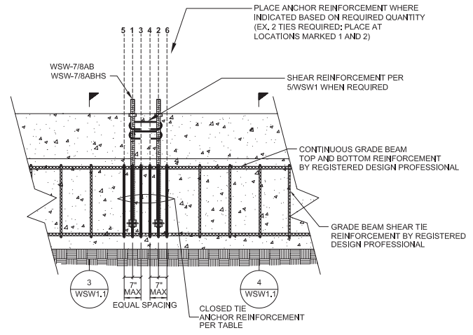
GRADE BEAM ELEVATION AT 12" AND 18" WALL MODELS
