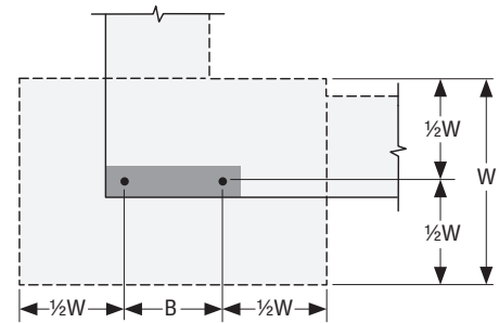
Footing Plan
