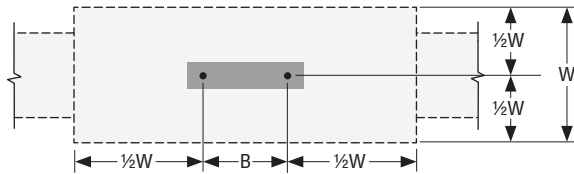
Footing Plan
