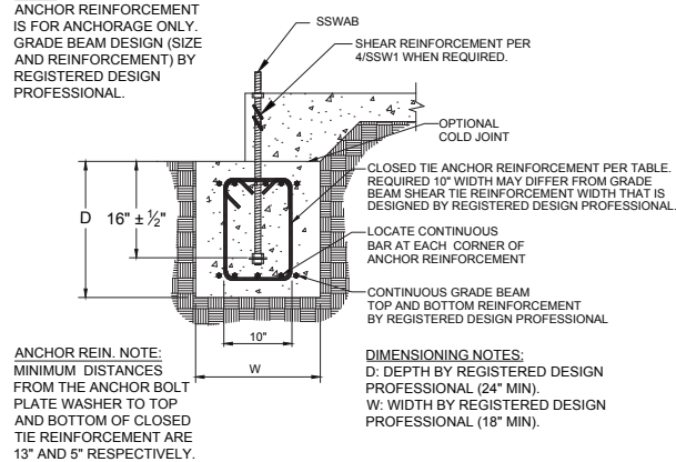
GRADE BEAM SECTION AT ANCHOR REINFORCEMENT
