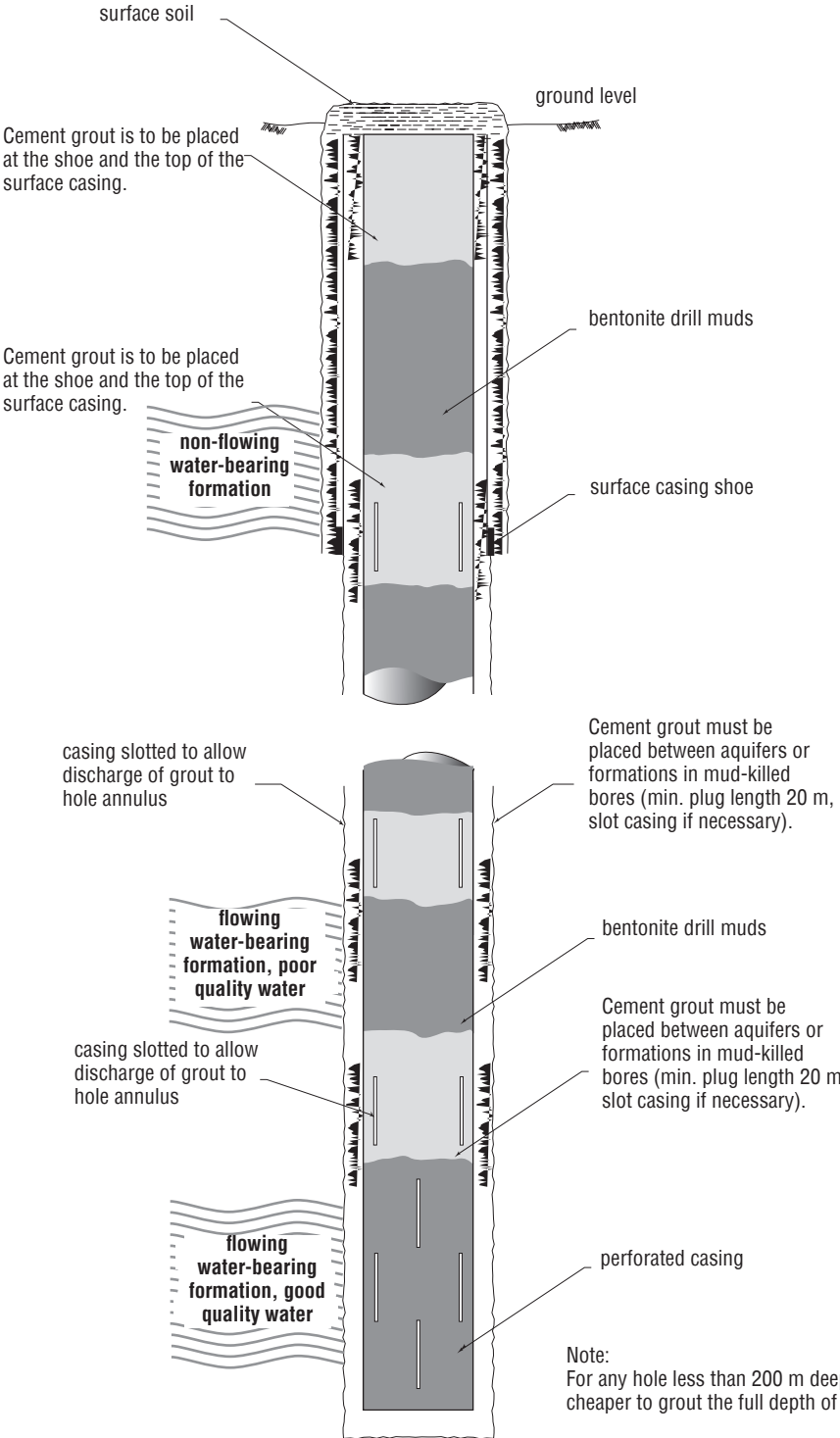
Figure 18.4 Decommissioning a flowing bore using cement grout bridges
