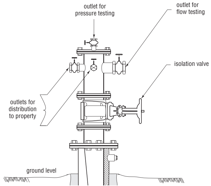
Figure 16.1 An example of headworks design for a flowing bore
