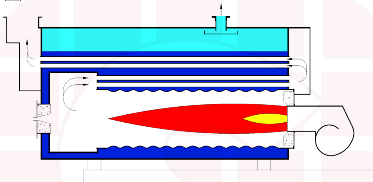
Graphic Depiction of 3-Pass Wetback Steam Pass Configuration
