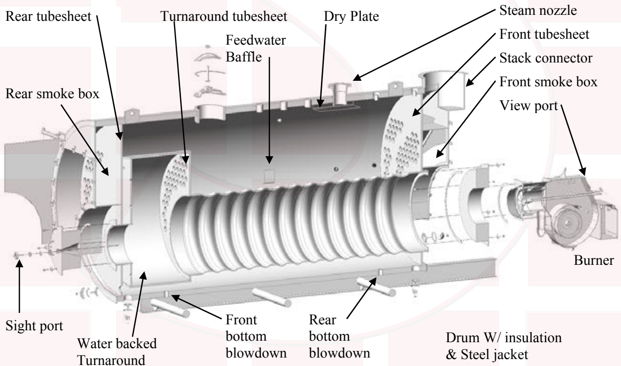
Steam boiler cross section: Figure 4
