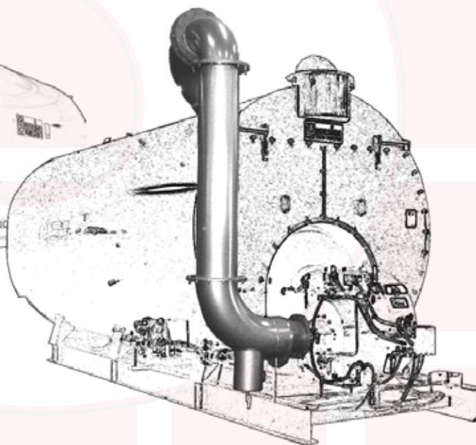
Example flue gas return (same boiler as fig 32): Figure 30
