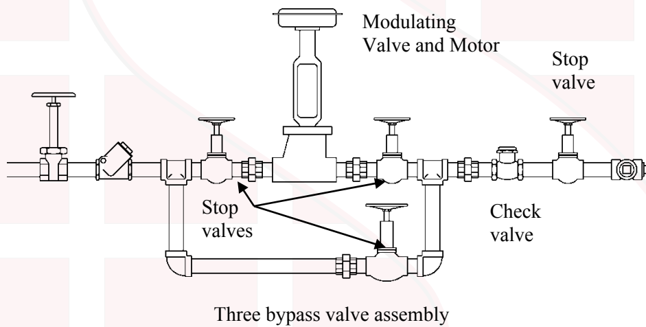
Example of feedwater piping with 3 valve bypass. Figure 22
