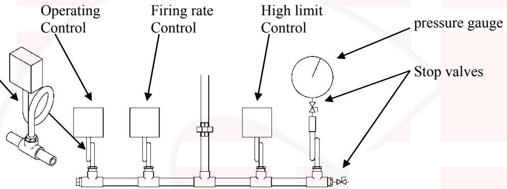
Typical pressure manifold, Figure 9
