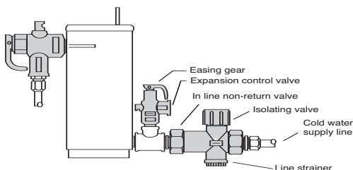
Fig 1.2 Typical installation mains pressure storage water heater with expansion control valve
