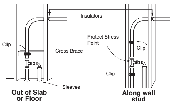
Fig 1.5 Pipe clipping
