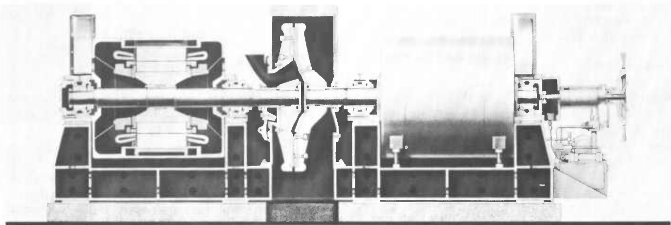
Figure 86 —Cutaway view of a double-revolving-disk mill (Bauer).
