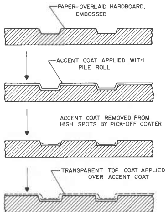
Figure 306 —Finishing sequence of paper-overlaid embossed hardboard.
