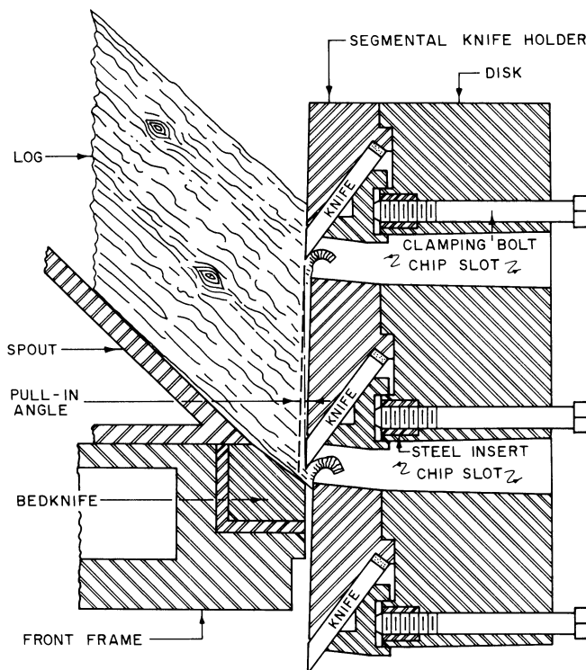
Figure 56 —Section through Carthage Norman type chipper, illustrating cutting action (Lamarche 1969).
