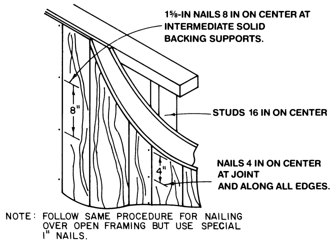
Figure 352 —Application of wall paneling over solid backing, such as plaster or gypsum board (Masonite Corp.).
