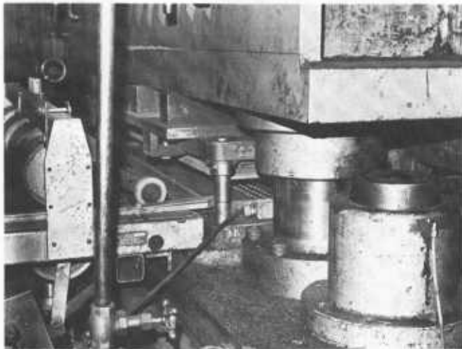
Figure 278 —Closeup of punch press showing bed plate and raised head with stripper plate. Advancement of panel and operation of punch proceed automatically.
