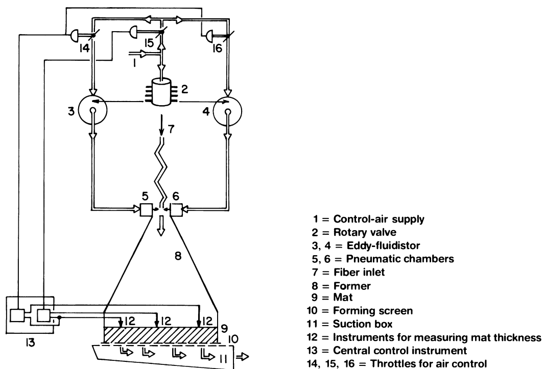
Figure 223 —Schematic drawing of Pendistor former (Carlson 1978).
