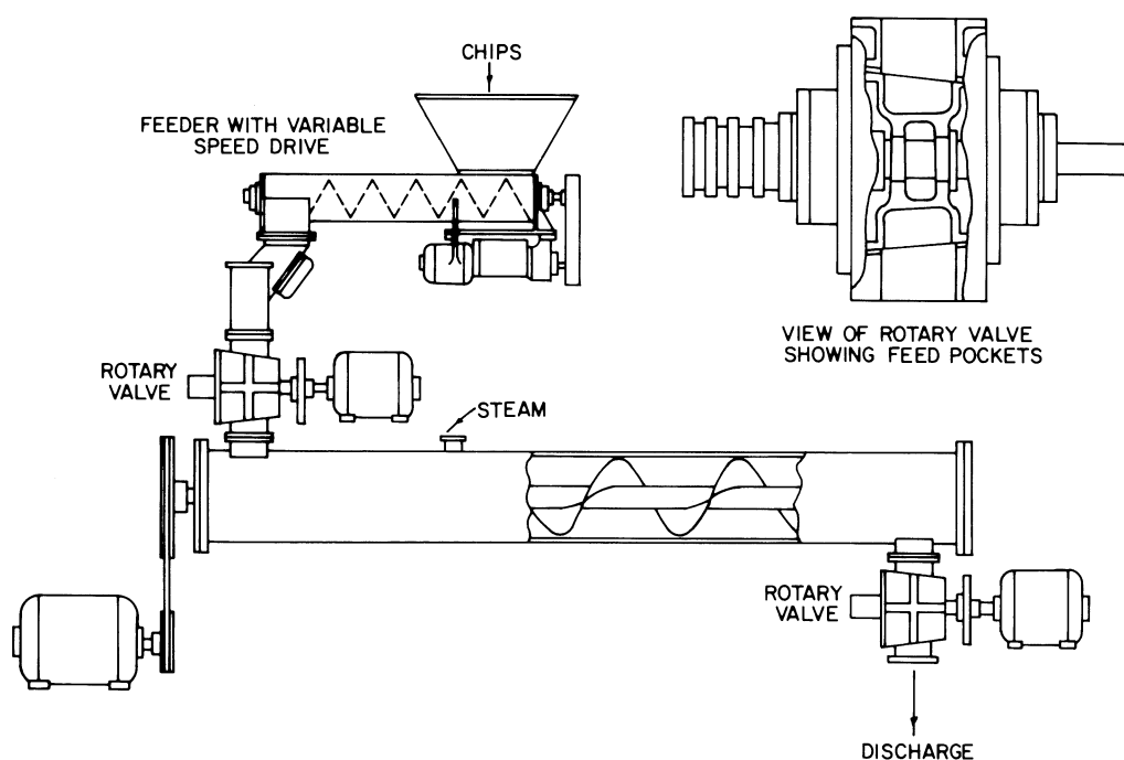
Figure 89—Grenco continuous digester (Atchison and Agronin 1958).
