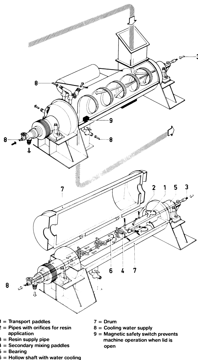
Figure 219 —Short retention mixer for particle furnish. Speed: 600 to 1,000 r/min (Bison Werke).
