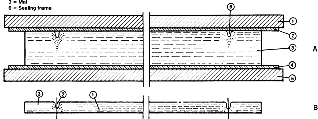
Figure 191 —Pressing of binderless hardboard (Swiderski 1963).
