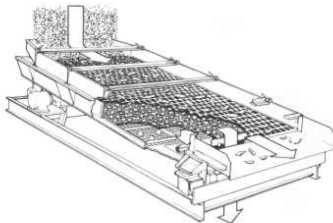
Figure 59—Rotex chip screener (Rotex).
