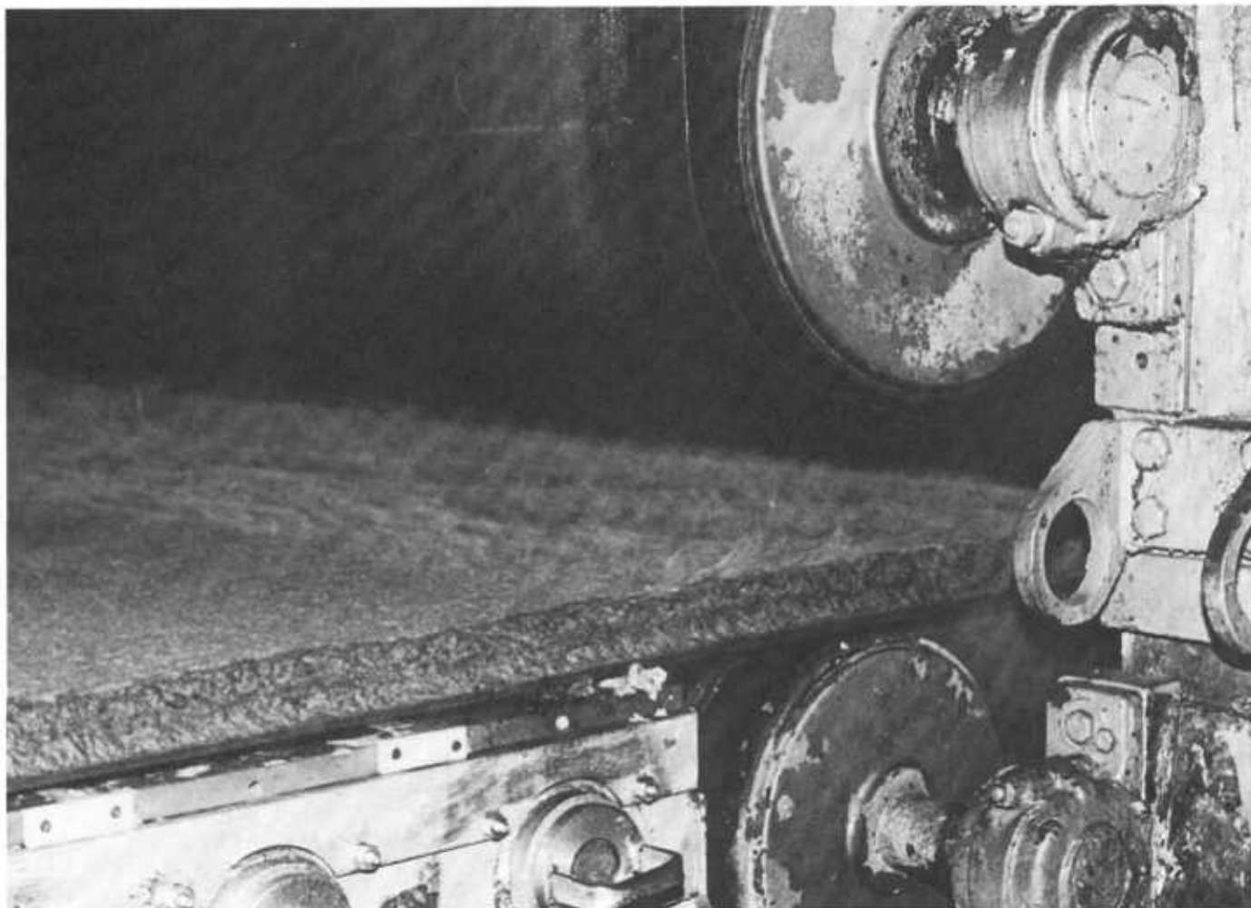
Figure 153—Infeed end of S1S wet press.
