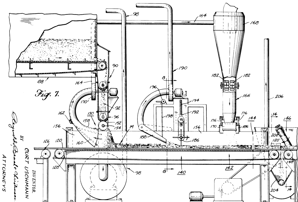
Figure 199—Patent drawing of forming machine used in Cascade Plywood Corporation board plant at Lebanon, OR (now Champion International) (Ushmann 1956).
