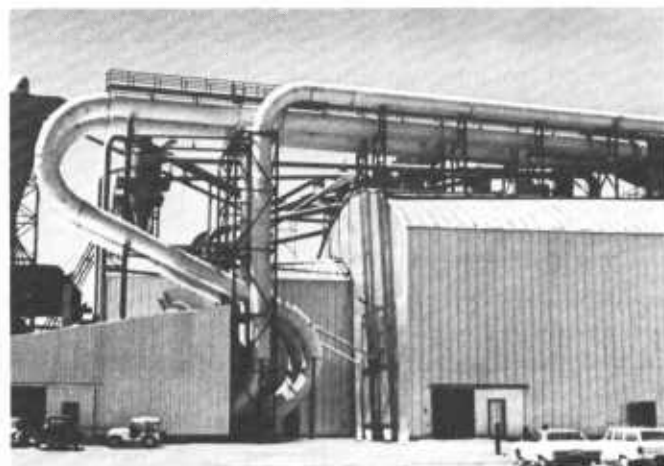
Figure 194 — Suspension tube flash-dryer in medium-density fiberboard plant (M-E-C Co.).
