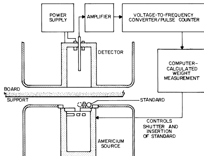
Figure 213—Principle of Measurex weight sensor (Betzner and Wallace 1980).
