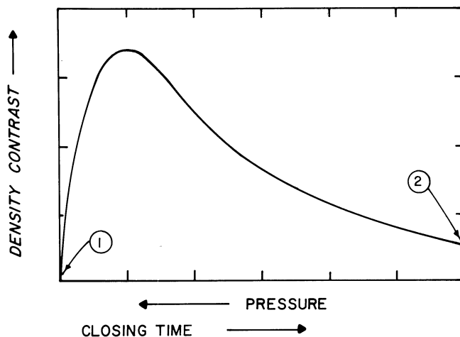
Figure 226 —Schematic illustration of relationship between pressure or closing time and density contrast over cross section of medium-density fiberboard (Suchsland and Woodson 1974).
