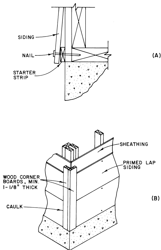
Figure 357 —Details of hardboard lap siding application (American Hardboard Association). Starter strip (A) and outside corner (B).
