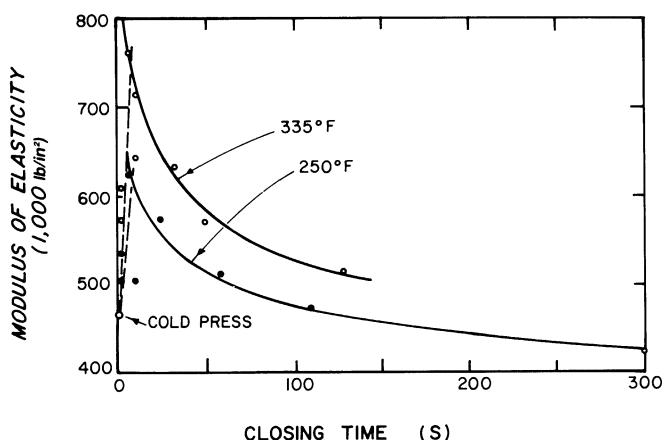
Figure 227 —Relationship between press closing time and modulus of elasticity in bending of experimental medium-density fiberboard pressed at two different platen temperatures (Suchsland and Woodson 1974).
