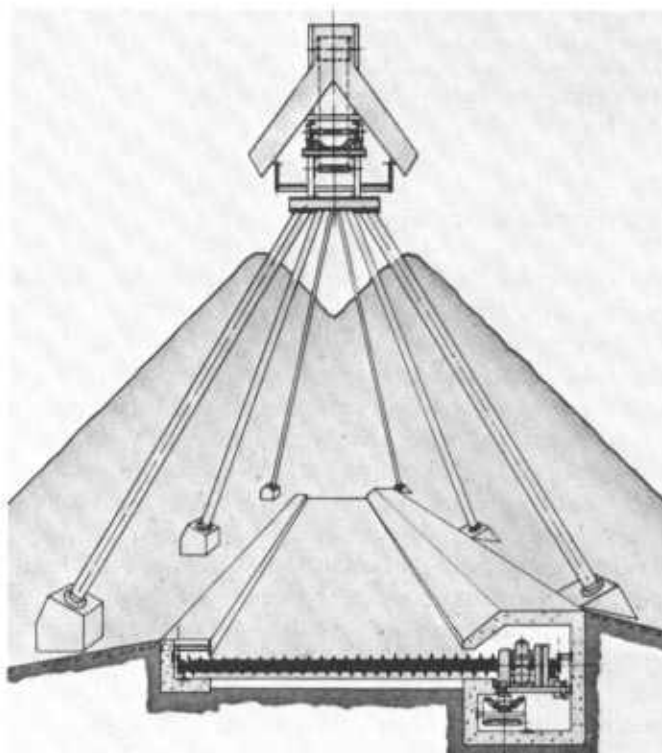
Figure 65 —Mechanical reclaimer system for long chip piles (K.M.W. Systems).
