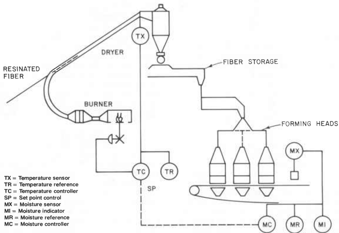
Figure 195—Fiber dryer controlled by dryer outlet temperature and mat moisture content (Chapman 1977).
