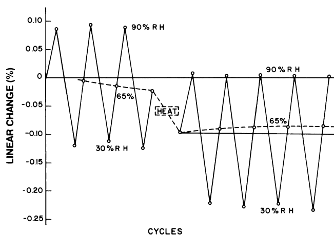
Figure 245 —Linear changes in response to cyclic exposure of 1/8-in hardboard before and after heat treatment at 375 °F for 2 1/2 h (Klinga and Back 1964).
