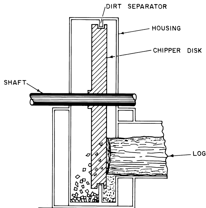
Figure 35—Principle of dirt separator of Morbark Chipharvestor (Morbark Industries).
