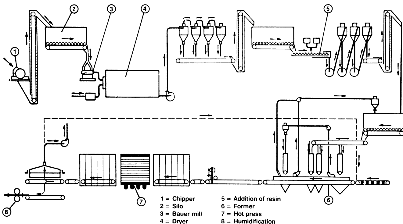
Figure 200—Schematic chart of dry-process hard-board plant of Cascade Plywood Company in Lebanon, OR (now Champion International) (Sandermann and Kunнемeyer 1957).
