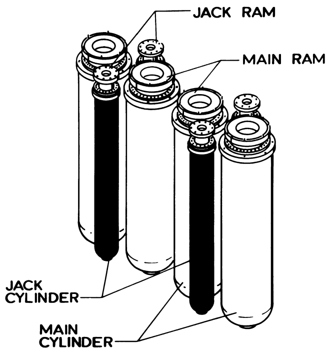
Figure 162 —Arrangement of jack and main rams in hydraulic press (Morse 1967). Small-diameter jack rams provide enough force to close press quickly without requiring large pump capacity. After press is closed, main rams apply high pressure with small travel without requiring large pump capacity.
