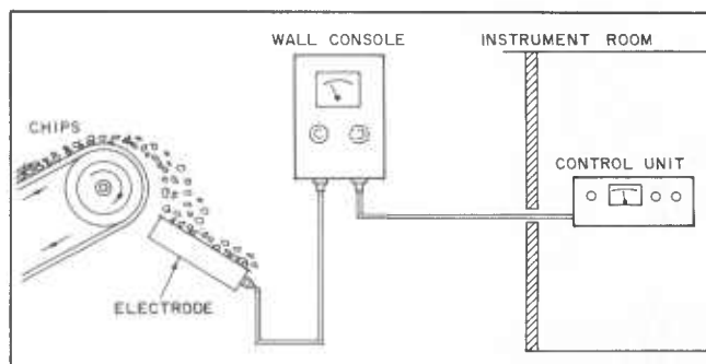
Figure 60—Schematic of continuous chip moisture content measurement (Lundstrom 1970). (© 1980 TAPPI. Reprinted from Tappi Journal , May 1980, pp. 857-861, with permission.)
