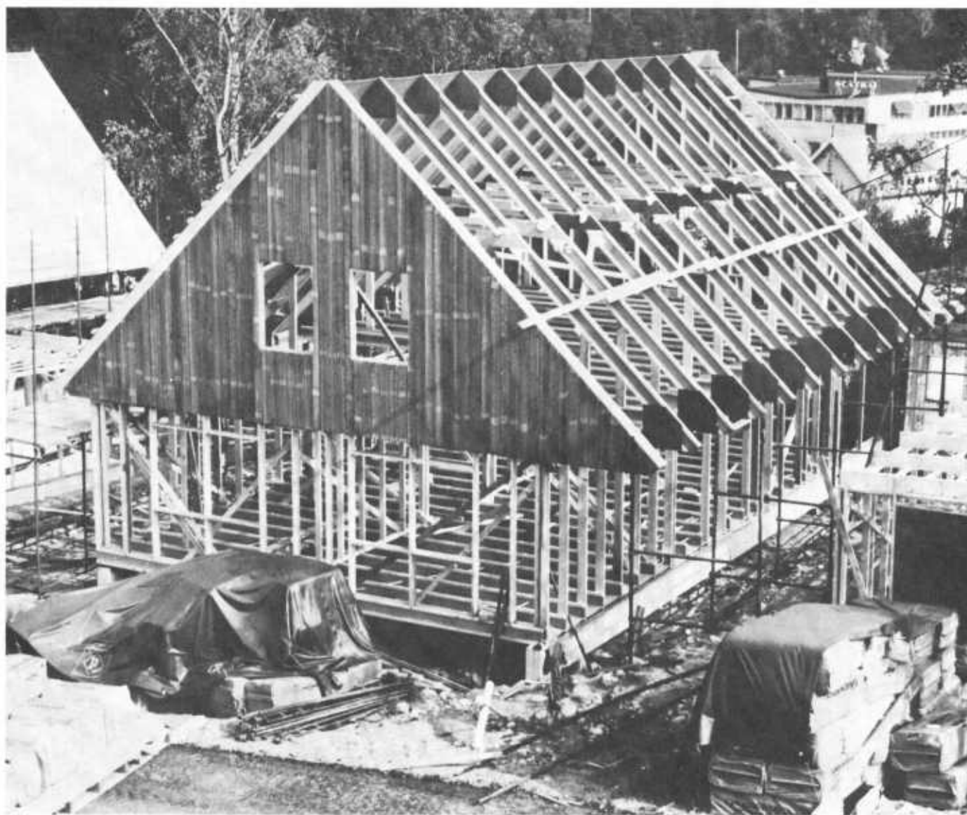
Figure 365 —Roof rafter system consisting of hardboard webbed I-beams connected by hardboard gusset plates (McNatt 1980).
