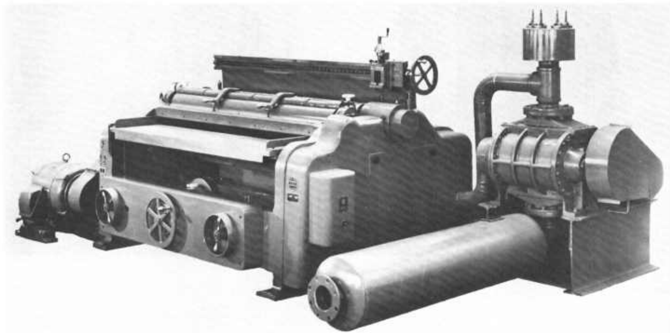
Figure 265 —Buss Micro Surfacers. A 52-in-wide single surfacer equipped with carbide knives and vacuum bed (note vacuum pump at right) (Buss).
