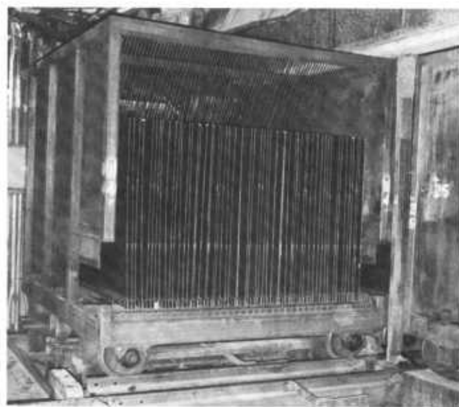
Figure 252 —Buggy loaded with hardboard ready to enter heat treating oven. Boards are standing on edge.
