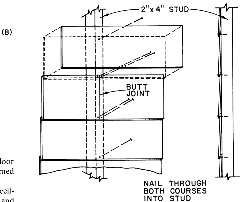
Figure 359 —Details of hardboard lap siding application showing joint at stud location (American Hardboard Association).
