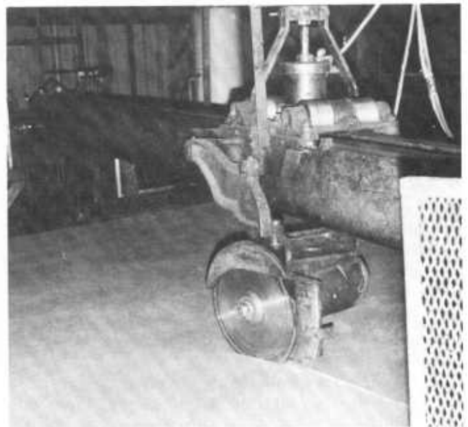
Figure 155 —Disk trimmer cutting traveling mat to length. Mat travel is from left to right. Overhead beam travels at same speed and in same direction as mat, while saw travels along beam across mat. When cut is completed the saw lifts up, and beam and saw return to initial position.
