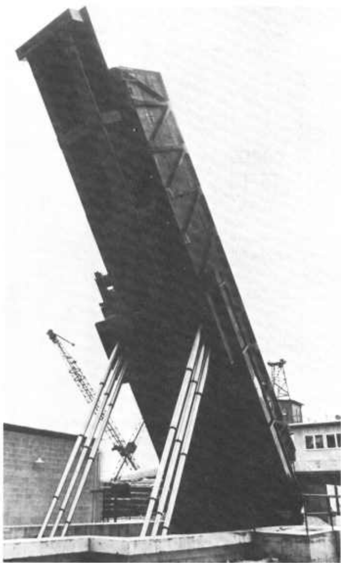
Figure 62 —A 300,000-lb-capacity rail car dumper (Peerless).
