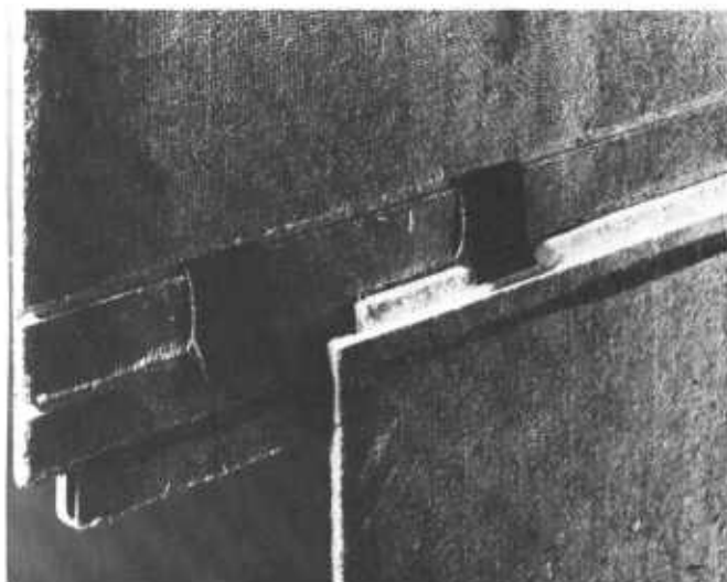
Figure 363 —Abitibi Random Shake Shingle Siding, System 25 clip (Abitibi-Price Corp.).
