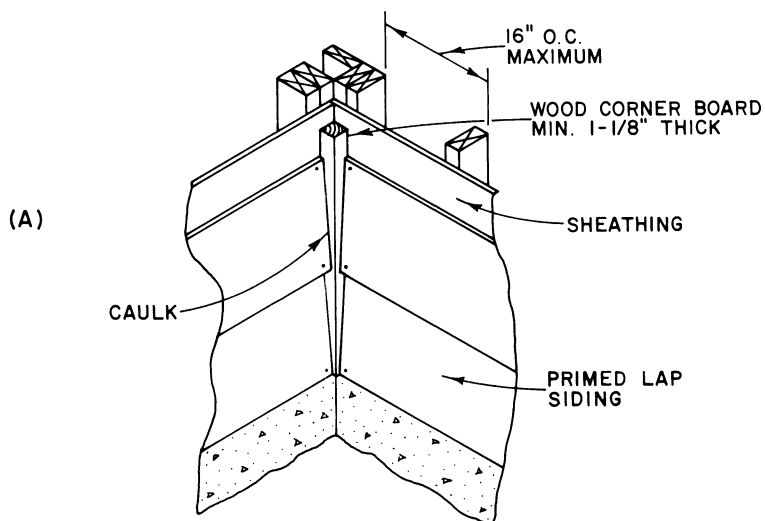
Figure 358 —Inside corner details of hardboard lap siding application (American Hardboard Association).
