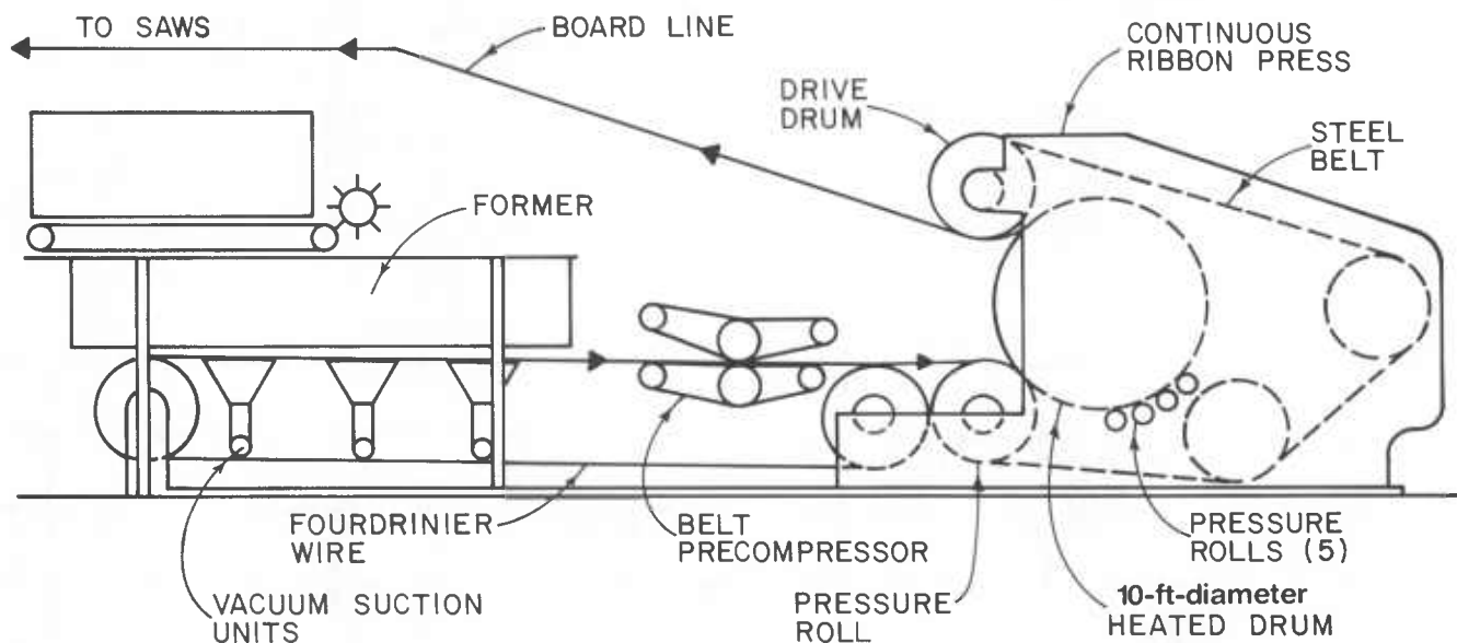
Figure 233 —Mende continuous press set up to press fiber mat (Wentworth 1971). Mat formed in former travels from left to right through precompressor and is then forced around heated drum by steel belt and pressure rolls.
