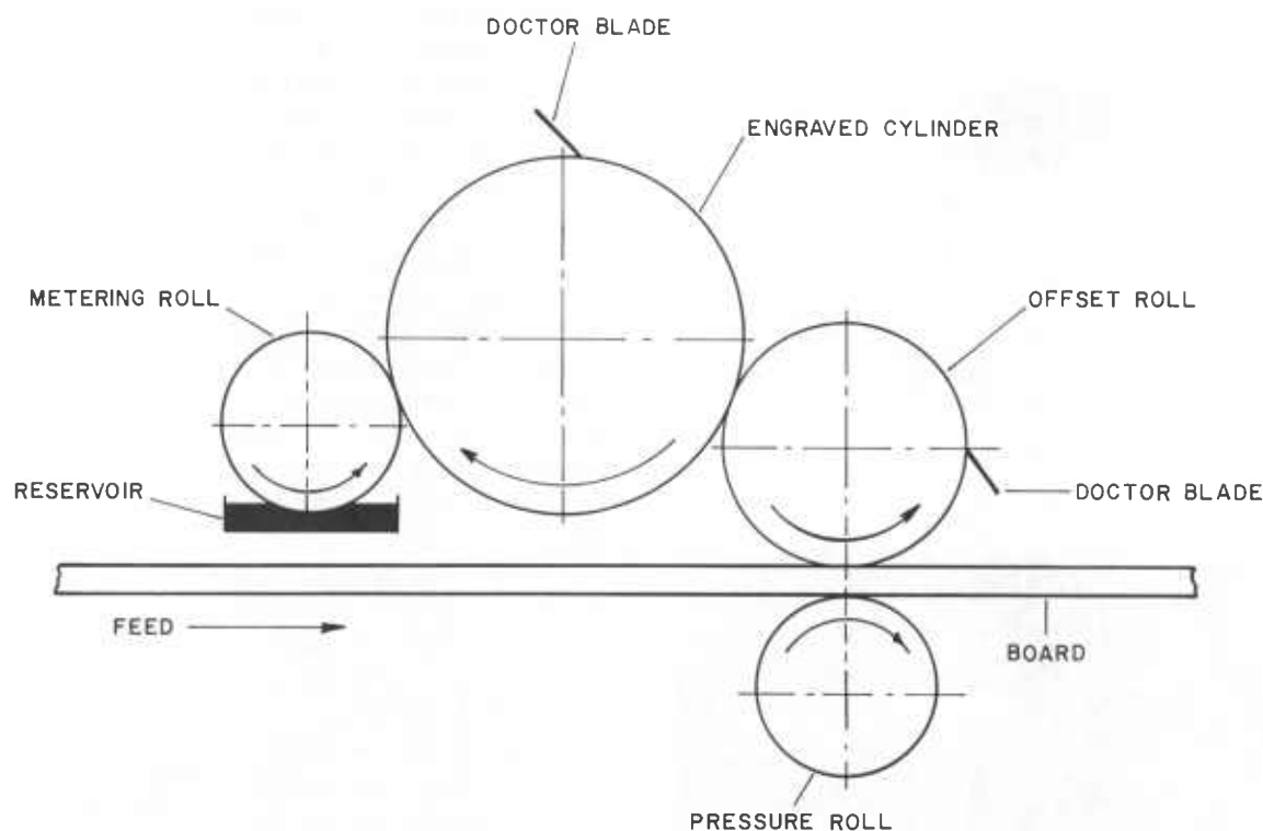
Figure 295—Schematic illustration of offset printer.
