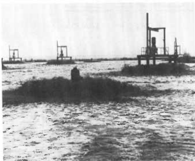
Figure 318 —Aeration lagoon with mechanical aerators.
