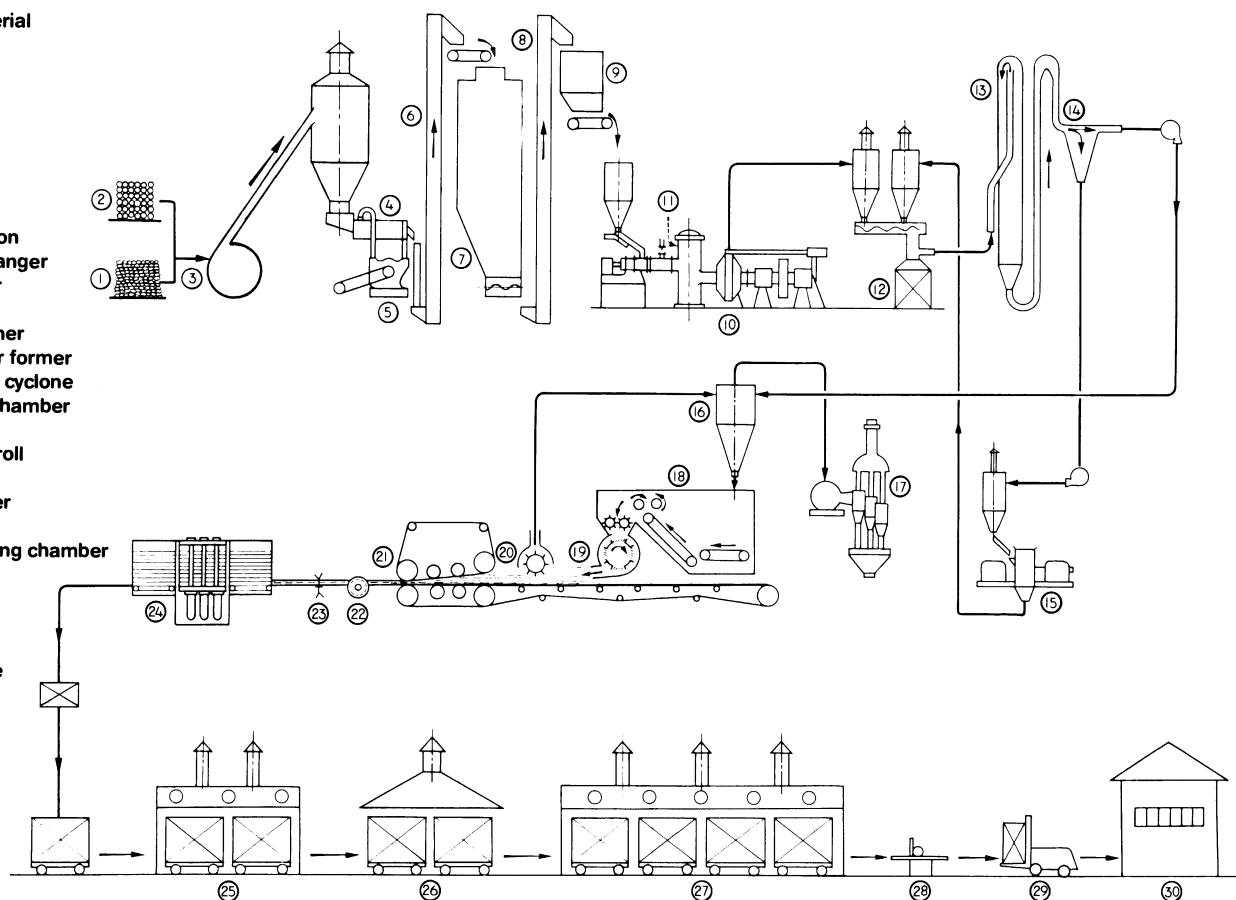
Figure 190 —Schematic process chart of Czechoslovakian binderless dry hardboard process (Swiderski 1963).
