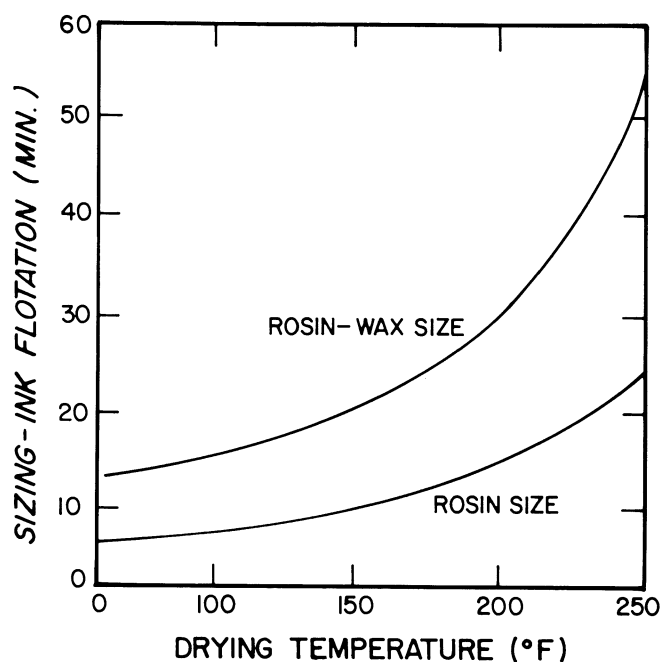
Figure 125 —Effect of drying temperature on the effectiveness of sizing as measured by the ink flotation test (longer time = better sizing) (Cobb and Swanson 1971). (© 1971 TAPPI. Swanson, T. W. Internal Sizing of Paper and Paperboard .)
