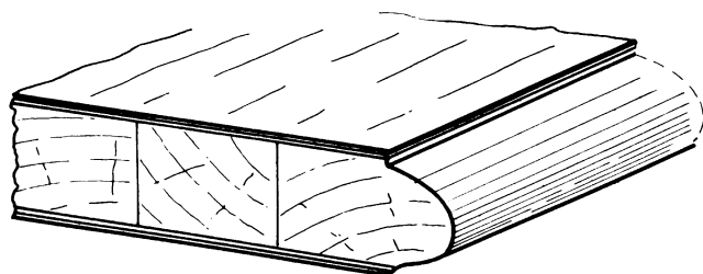
5 - PLY
