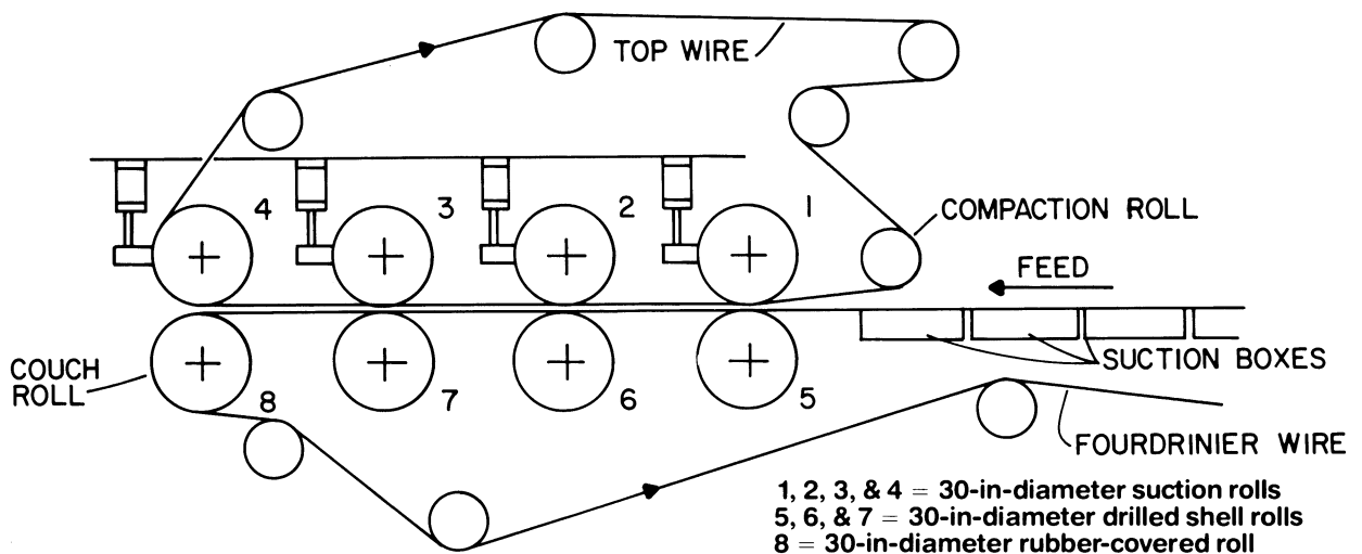
Figure 148—Wet-press section of insulation board machine.
