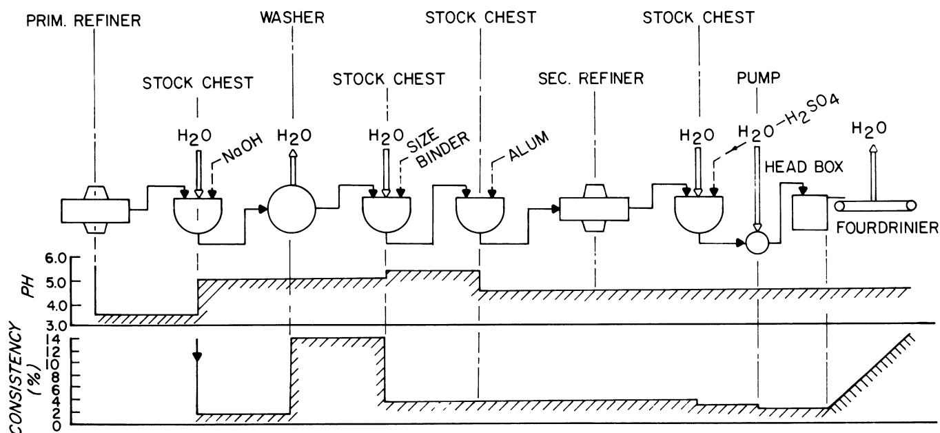
Figure 127 —Schematic of stock flow in wet-process fiberboard plant, showing pH, stock consistency, and introduction of additives.
