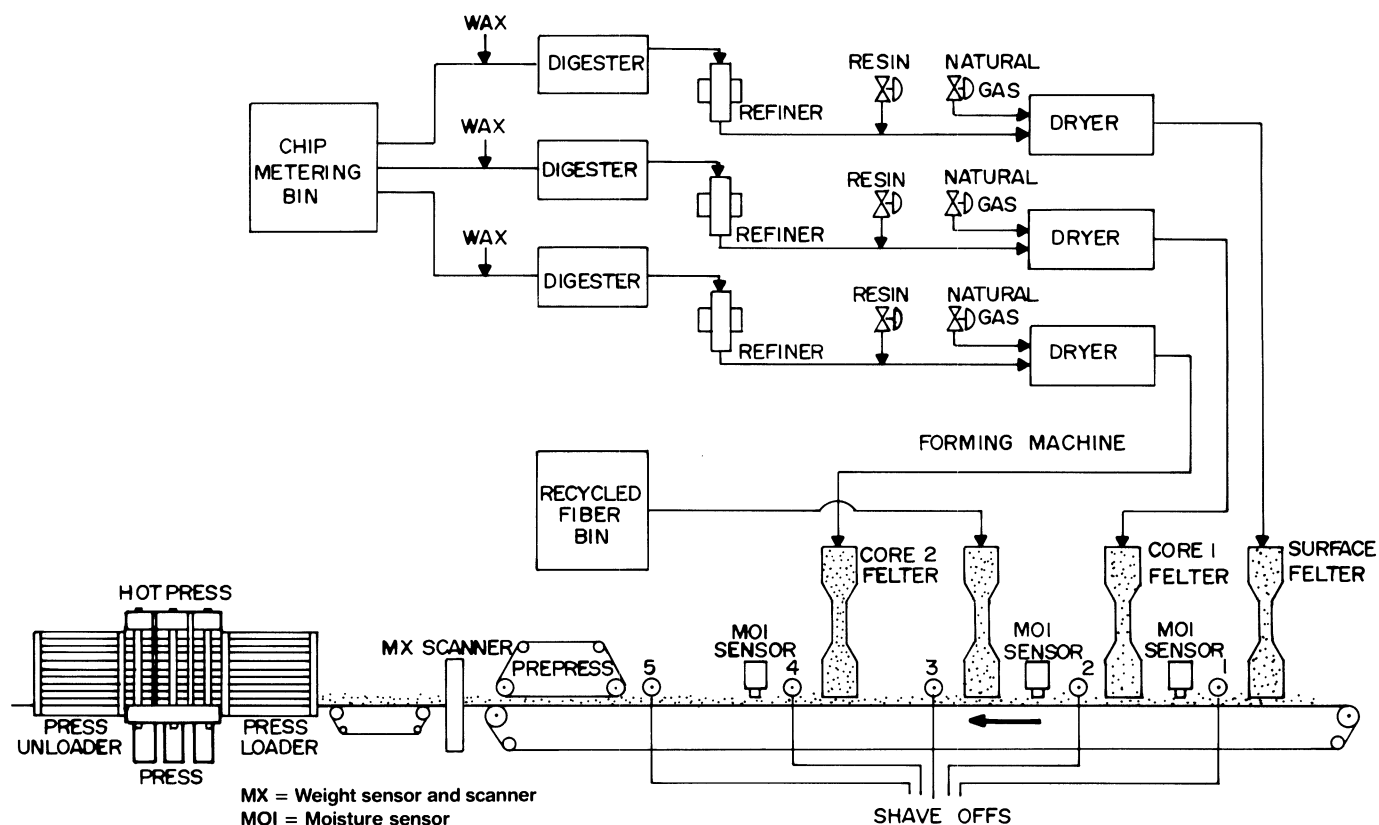
Figure 210—General schematic of hardboard siding line at Paris, TN (Beitzner and Wallace 1980).
