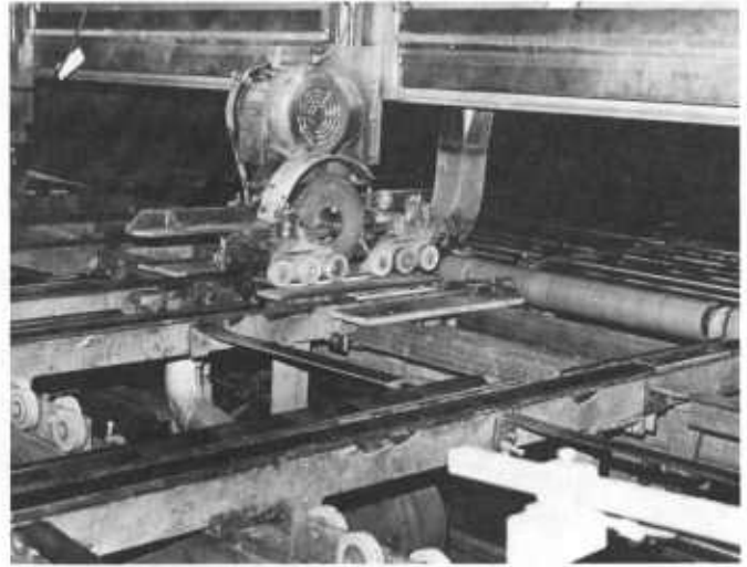
Figure 270 —Cross trimmer saw unit with individual drive for easy positioning along overhead beam.
