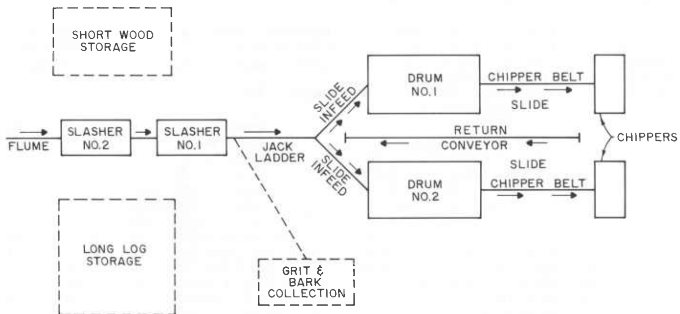
Figure 42 —Material flow in woodyard of pulp mill (Gilmer 1977).
