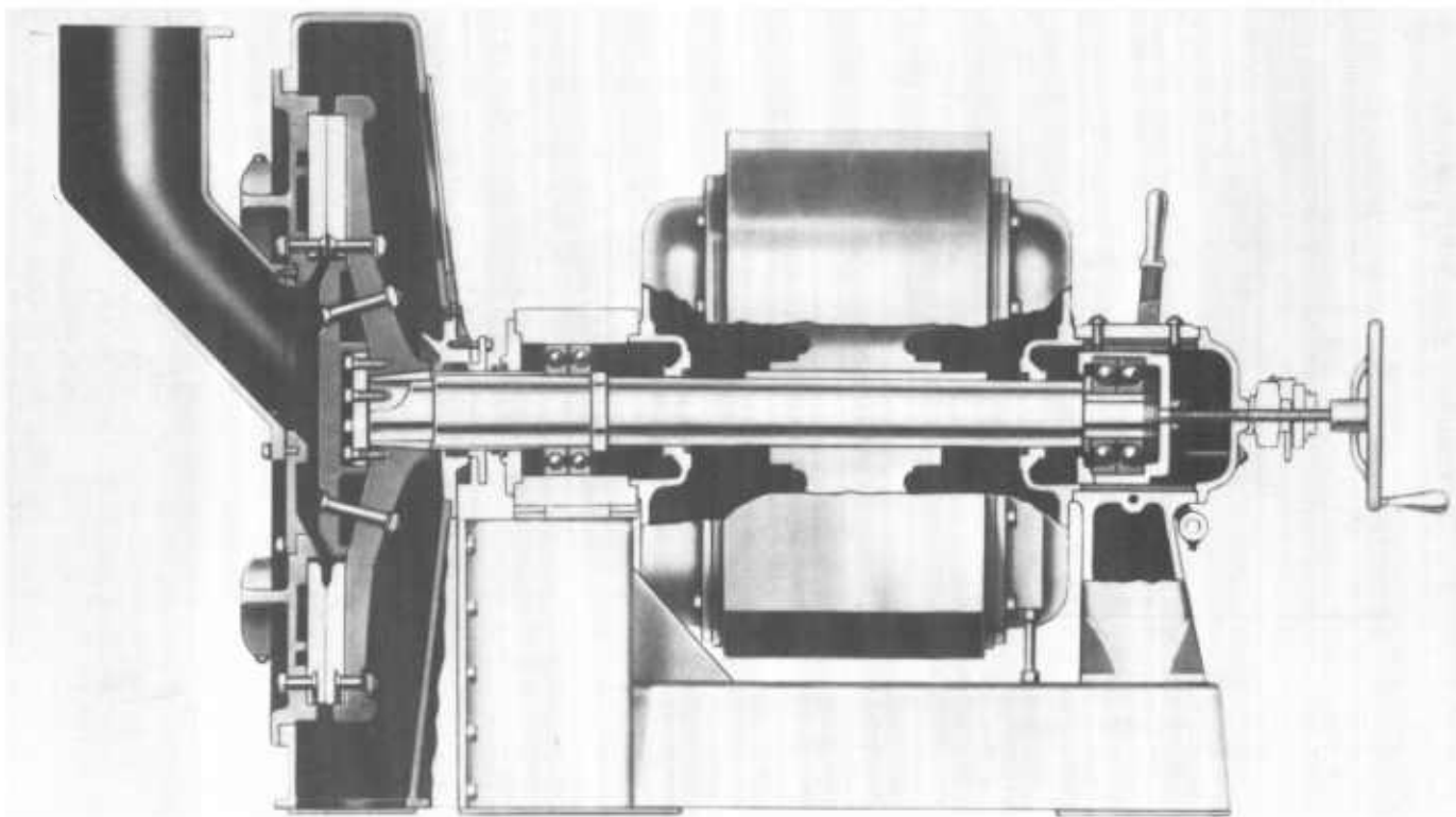
Figure 85 —Cutaway view of a single-revolving-disk mill (Bauer).
