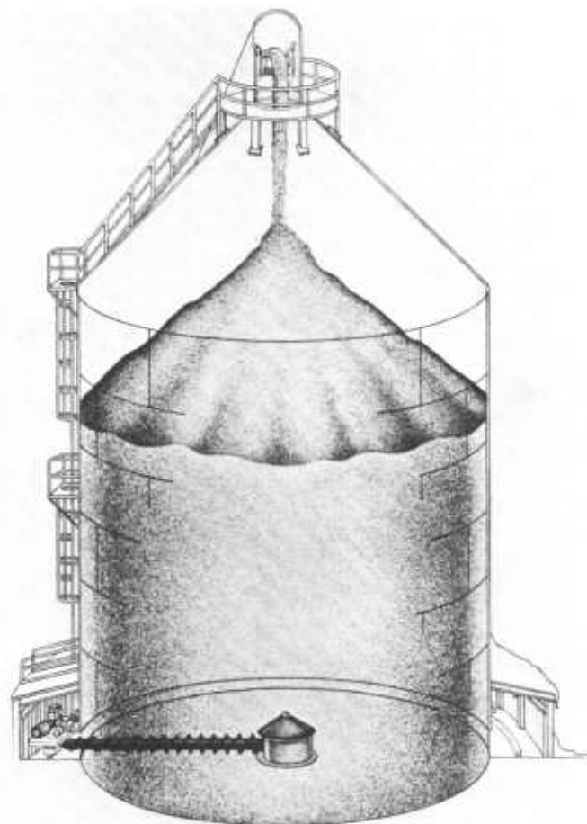
Figure 67 —Mechanical reclaimer system for circular chip piles and silos ( K.M.W. Systems ).
