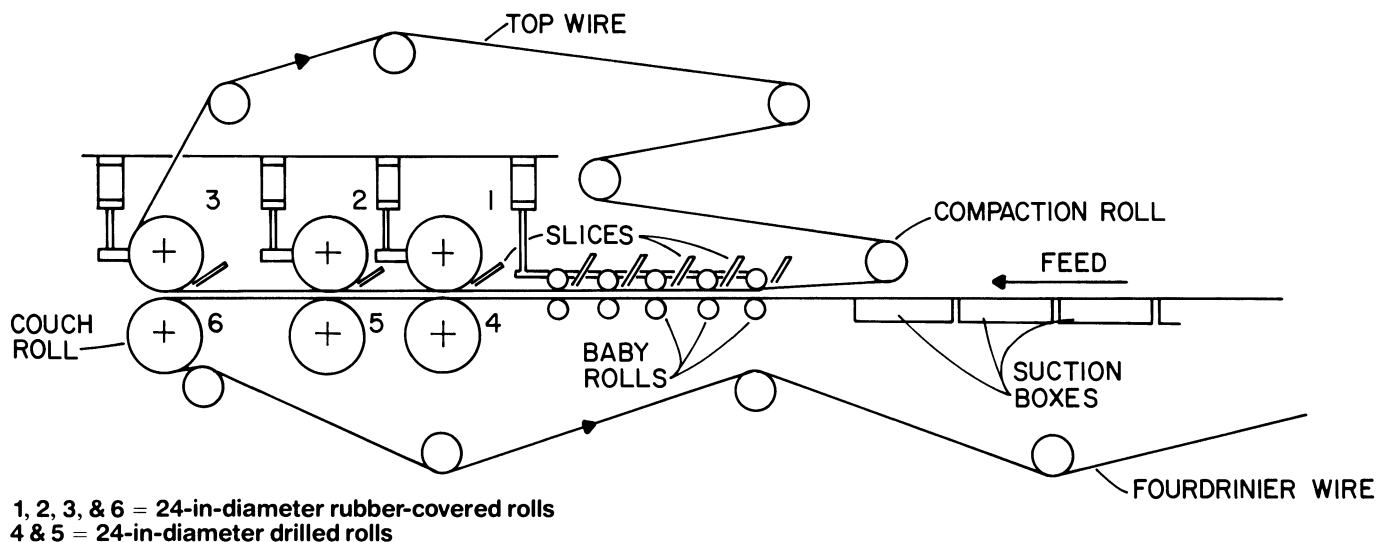
Figure 149—Wet-press section of hardboard machine.
