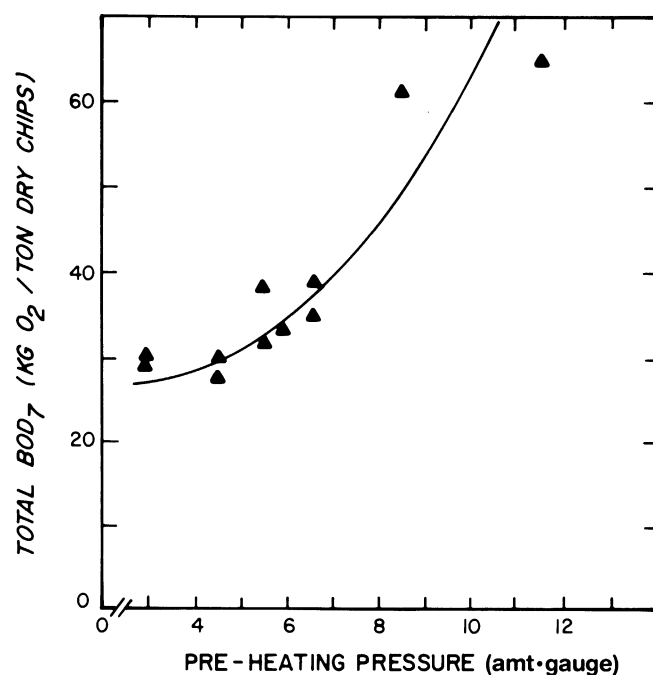
Figure 309 —Variation of BOD 7 with chip preheating pressure (EPA 1978).
