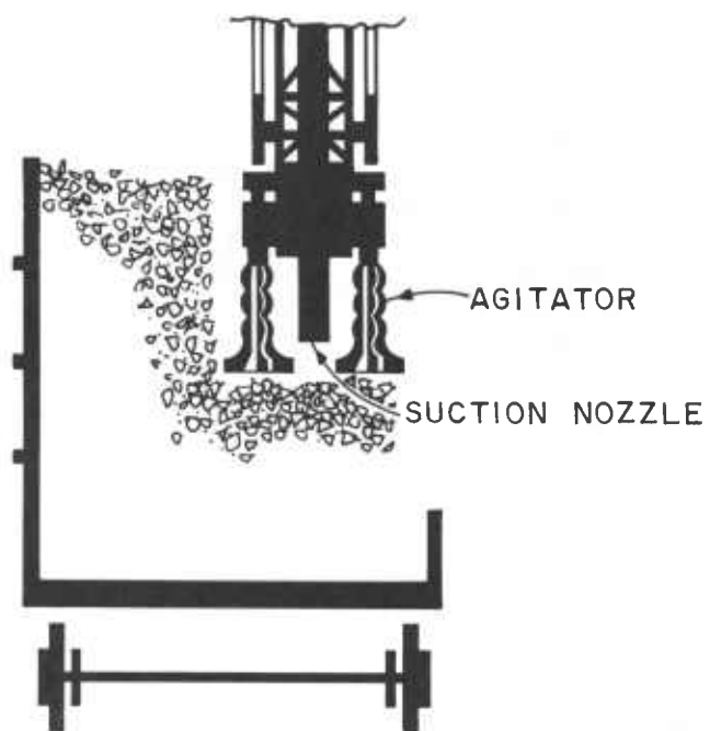
Figure 64 —Principle of open-top car vacuum unloader (Rader).
