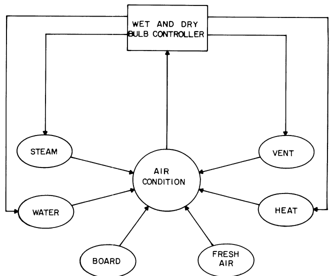
Figure 258 —Schematic of humidifier control.
