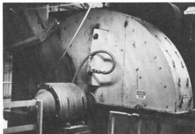
Figure 54 —A 116-inch gravity feed chipper carrying 16 knives, with a 1,000-hp motor.
