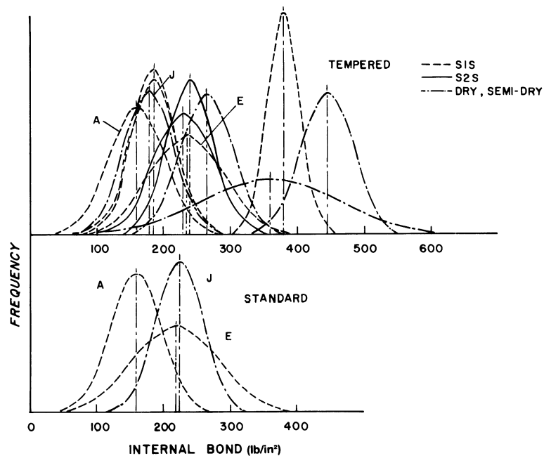
Figure 332 —Tensile strength perpendicular to surface (internal bond) of 1/4-inch hardboard types commercially manufactured in the United States (drawn from data by Werren and McNatt 1975). Letters refer to specific manufacturing plants.
