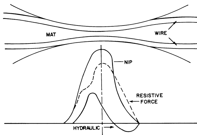
Figure 150—Internal mat pressure in press roll nip (Edge Wallboard).
