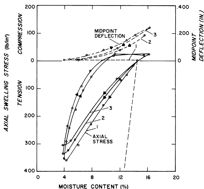
Figure 344 —Axial stresses and midpoint deflection of axially restrained hardboard strips as functions of moisture content (clamped wet) (Suchsland 1965). Numbers 1, 2, and 3 indicate sequence of exposure cycles. Dashed line represents theoretical stresses (assumption of elasticity).
